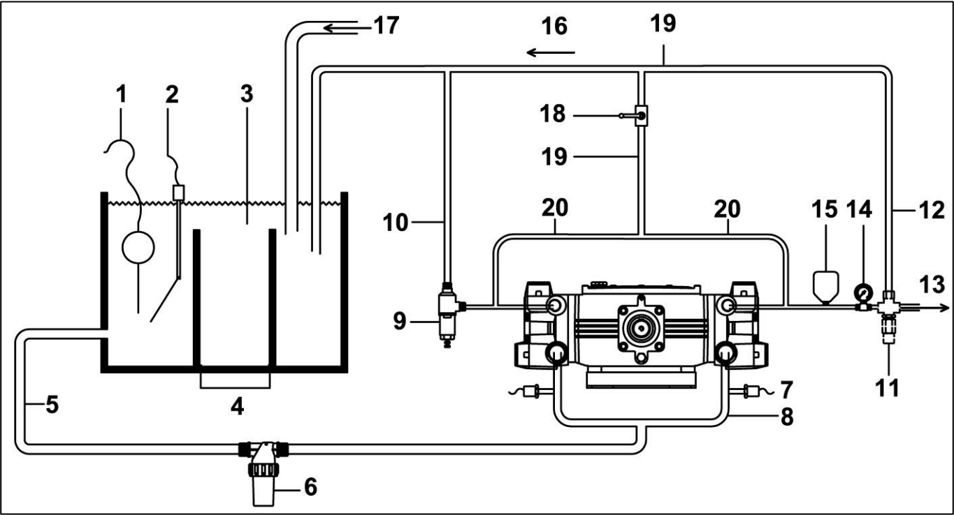
TYPICAL INSTALLATION FOR PUMPS C 3006
