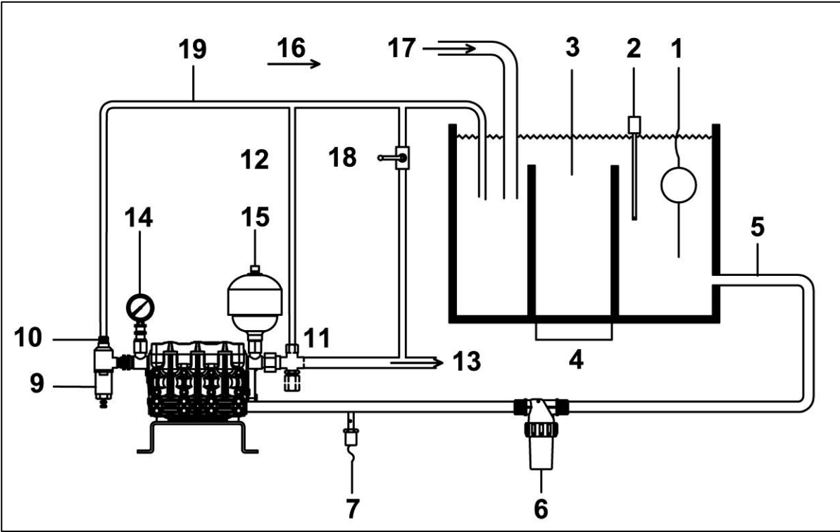
TYPICAL INSTALLATION FOR PUMPS CK 3003-CA 316-CPQ
